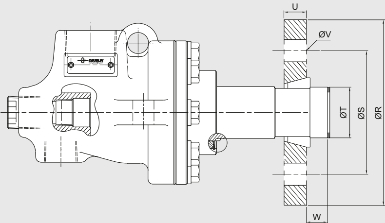
Quick Release Connection BC-54XXX-XX-32
