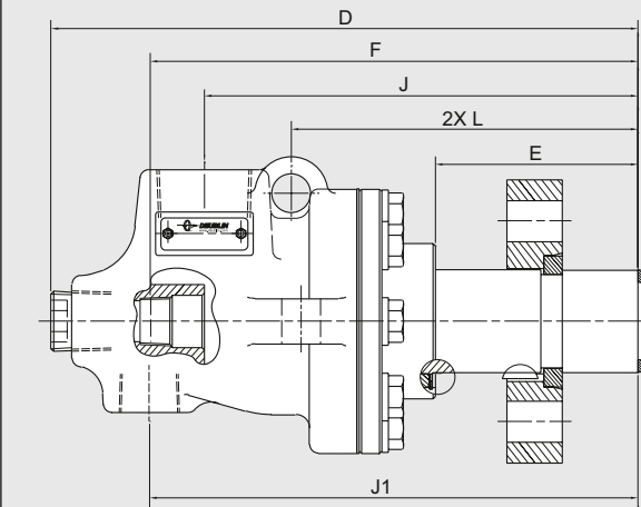
“CF” Connection BC-54XXX-XX-30
