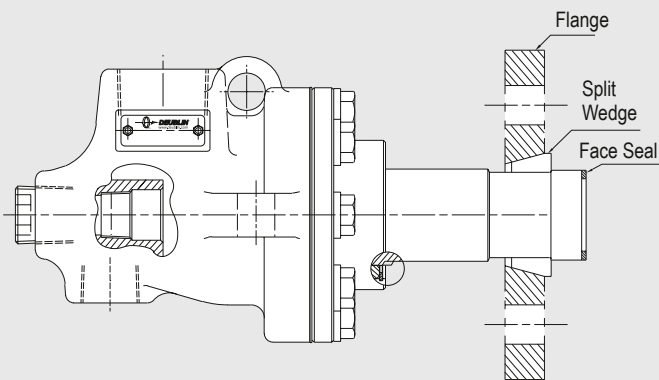
Quick Release Connection BC-54XXX-XX-32
