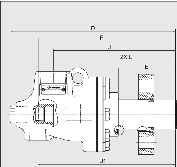
“CF” Connection BC-54XXX-XX-30
