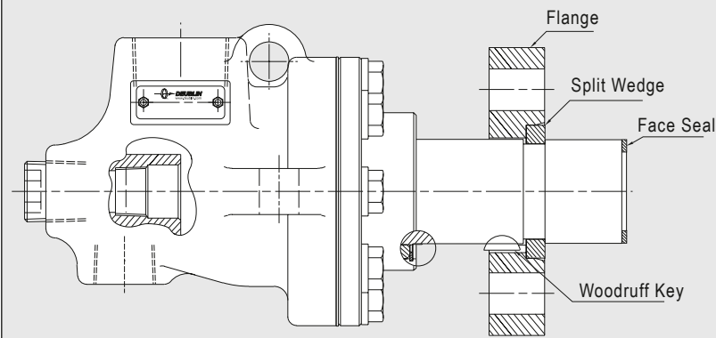
“CF” Connection BC-54XXX-XX-30
